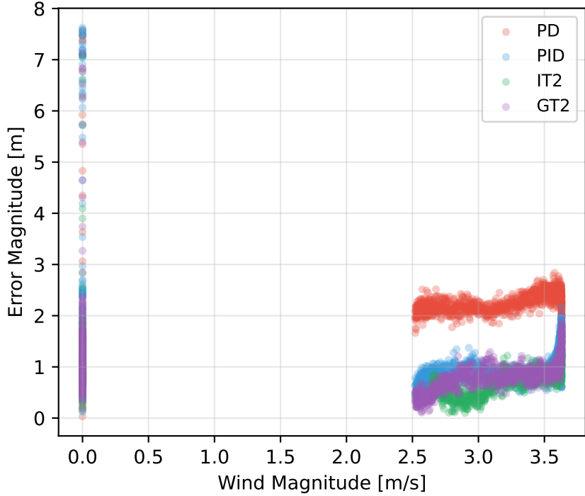
Wind vs Error Correlation - Phase 3
