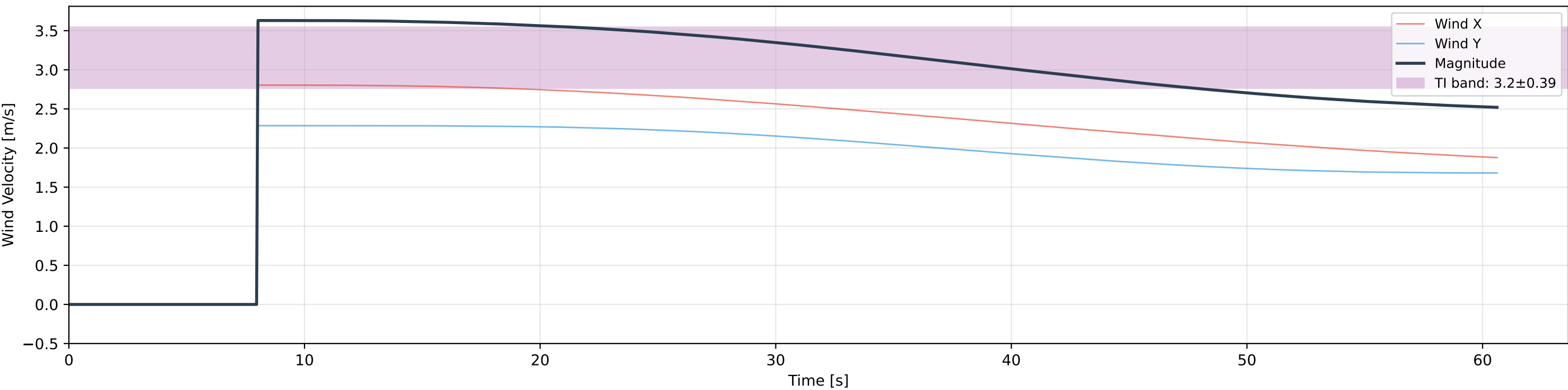
Wind Disturbance Profile - Phase 3 (TURBULENCE)
