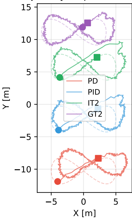
2D Trajectory (Top View) - Phase 3
