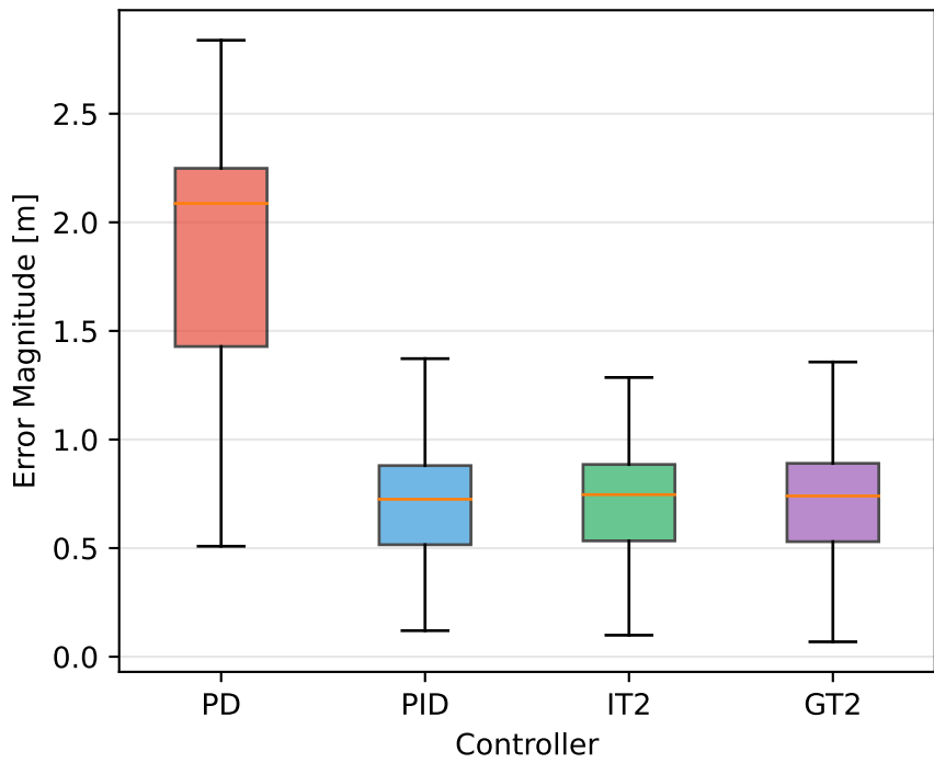
Steady-State Error Distribution - Phase 3
