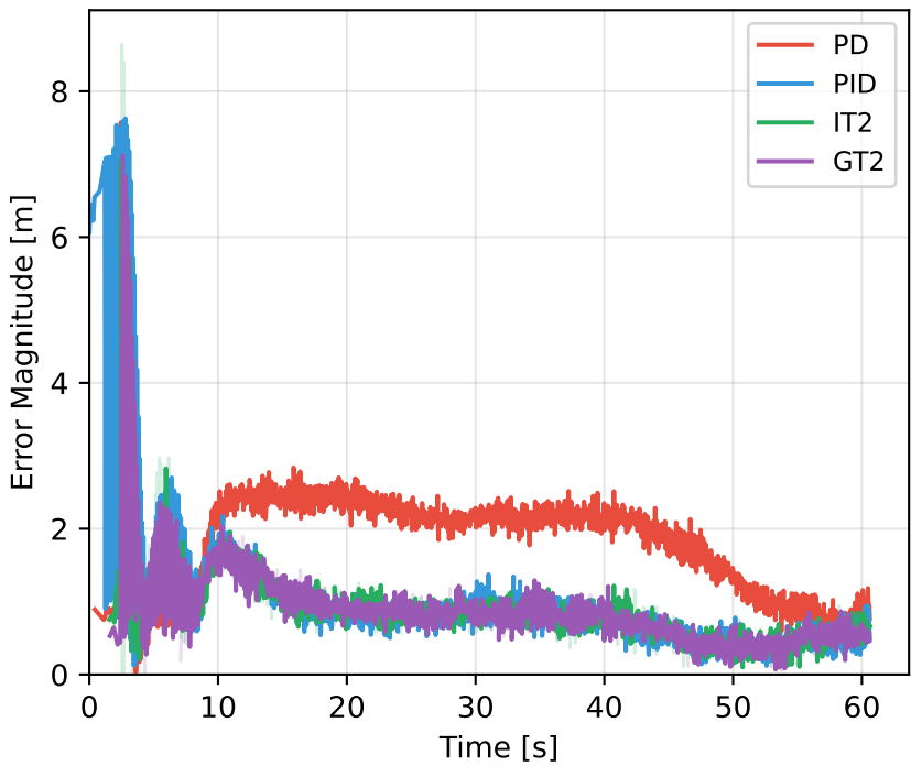
RMSE Evolution - Phase 3 (TURBULENCE)
