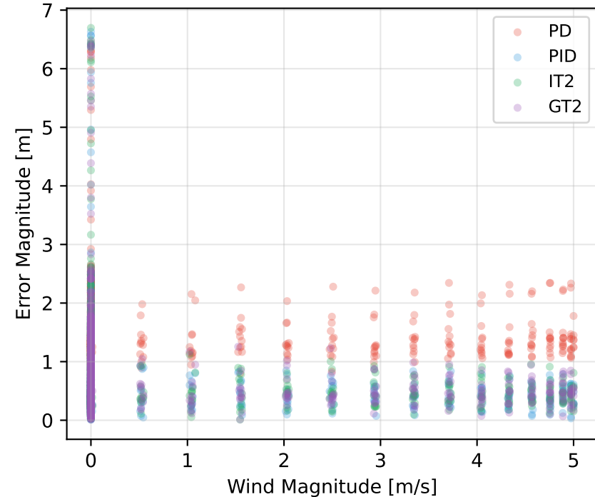
Wind vs Error Correlation - Phase 4
