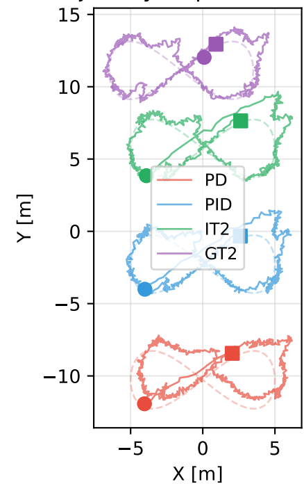
2D Trajectory (Top View) - Phase 4
