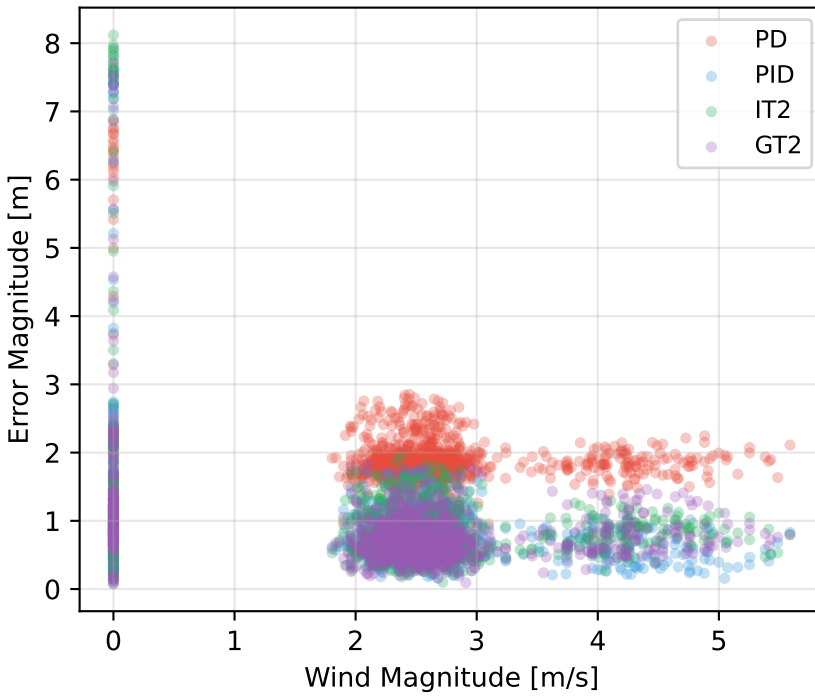
Wind vs Error Correlation - Phase 5
