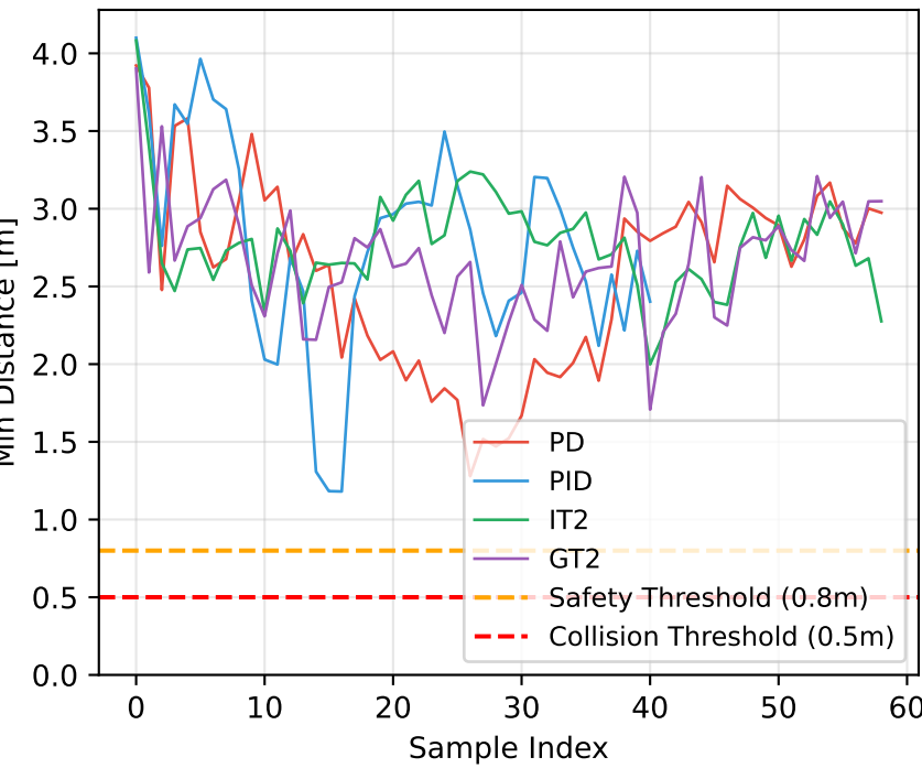
Min Inter-Agent Distance - Phase 5
