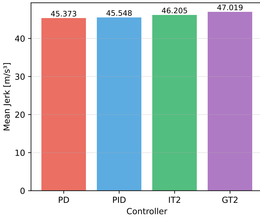
Jerk Analysis (Smoothness) - Phase 5
