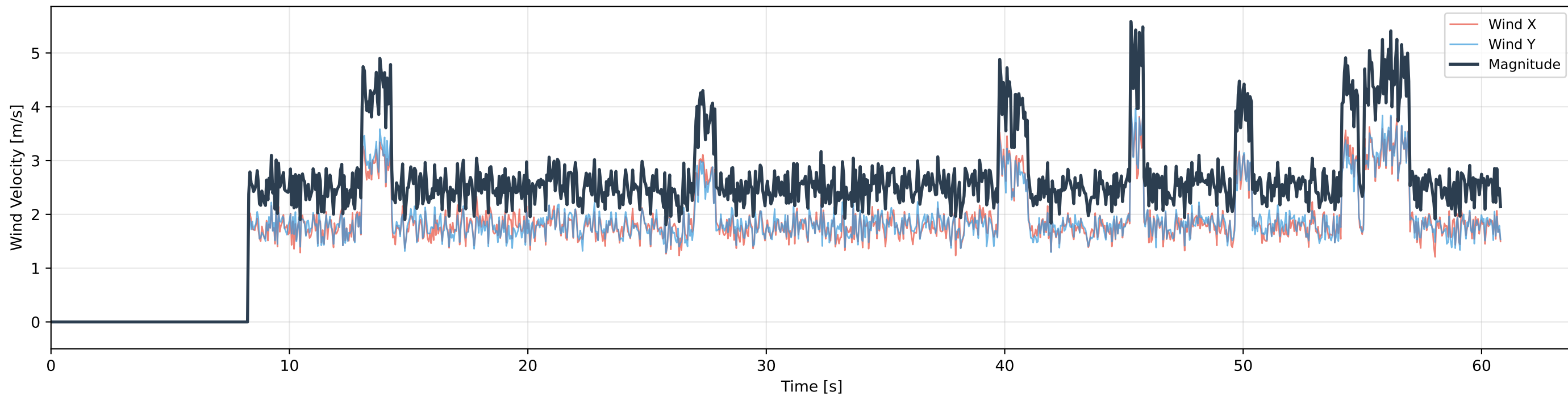
Wind Disturbance Profile - Phase 5 (COMBINED)
