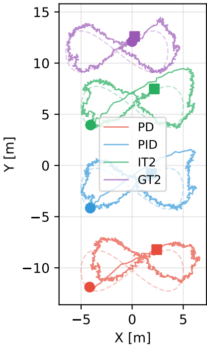
2D Trajectory (Top View) - Phase 5
