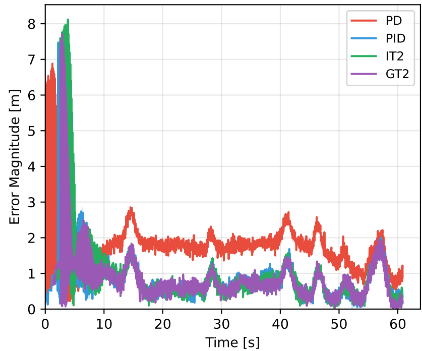
RMSE Evolution - Phase 5 (COMBINED)
