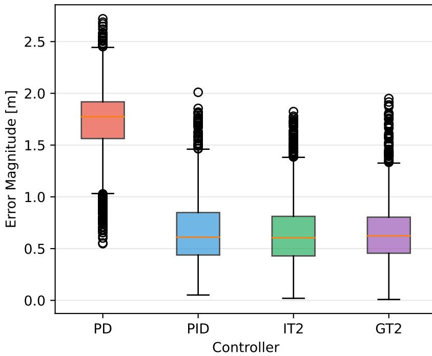
Steady-State Error Distribution - Phase 5
