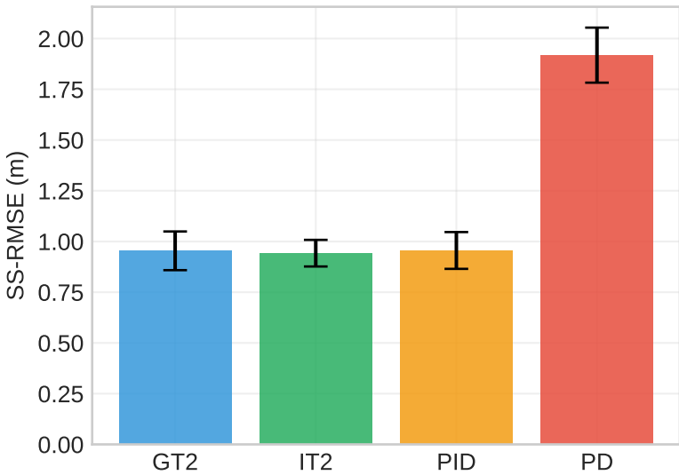
Steady-State RMSE
