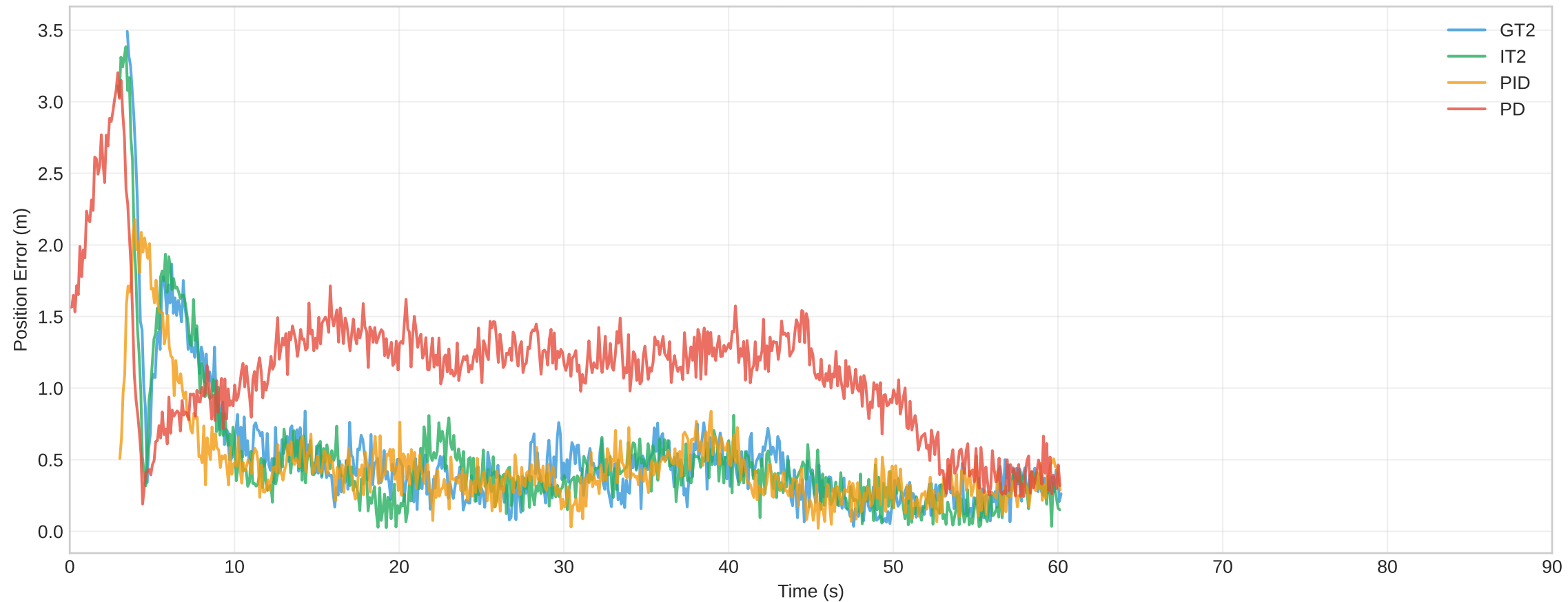
Phase 1: Baseline (No Wind) - Error Evolution
