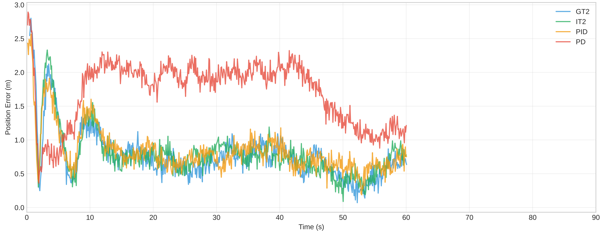
Phase 2: Steady Wind (3 m/s) - Error Evolution
