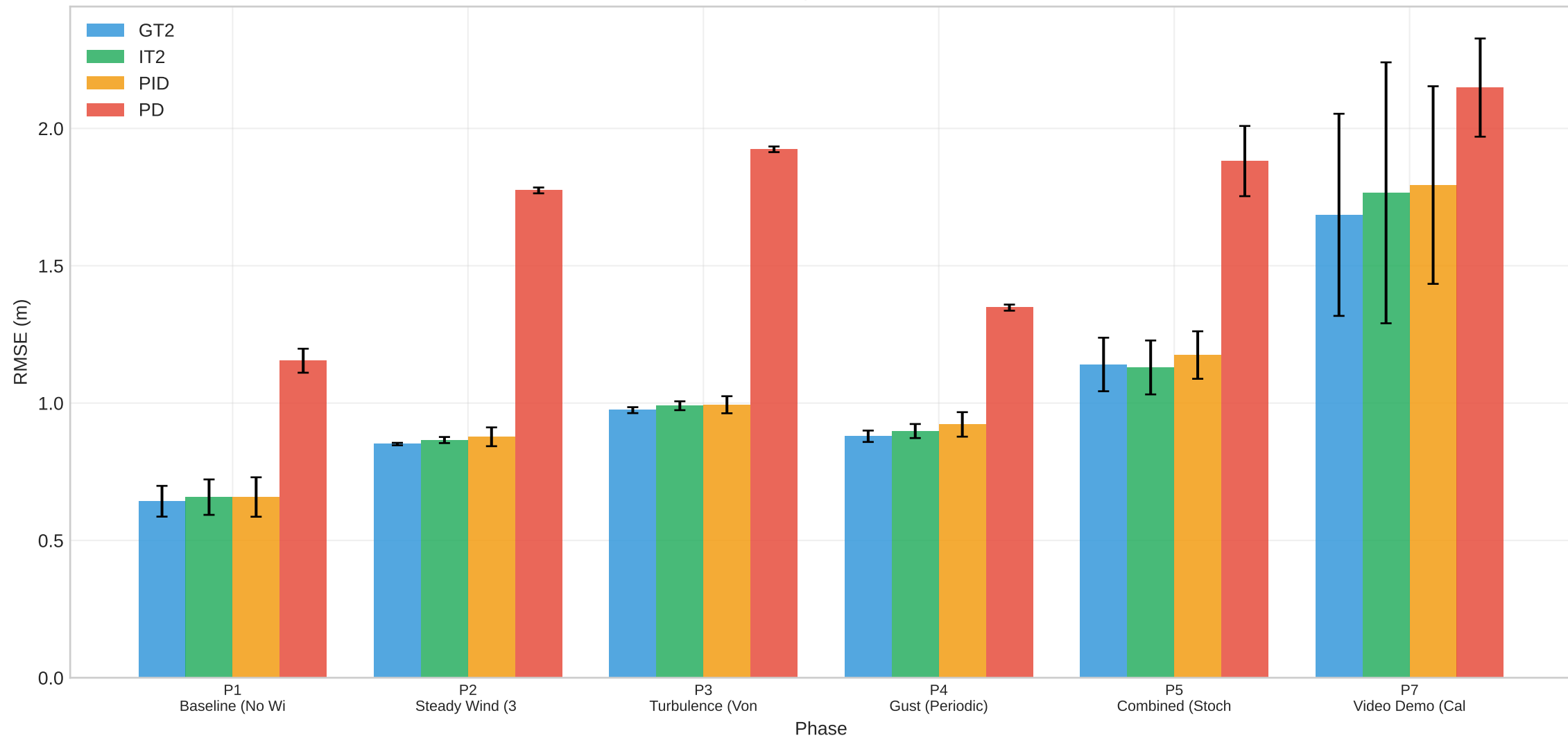
Controller RMSE Comparison Across All Phases
