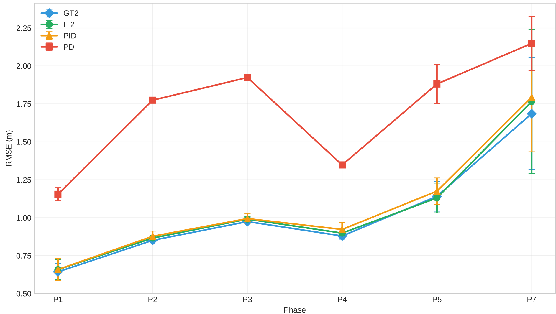
Controller Performance Trend Across Phases
