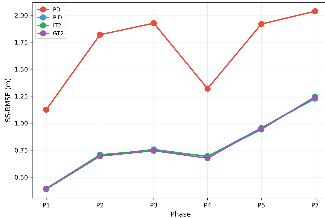
Steady-State RMSE Across Phases
