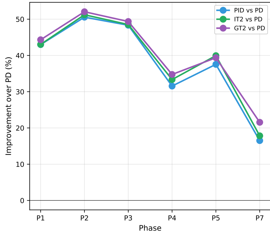
Controller Improvement over PD Baseline
