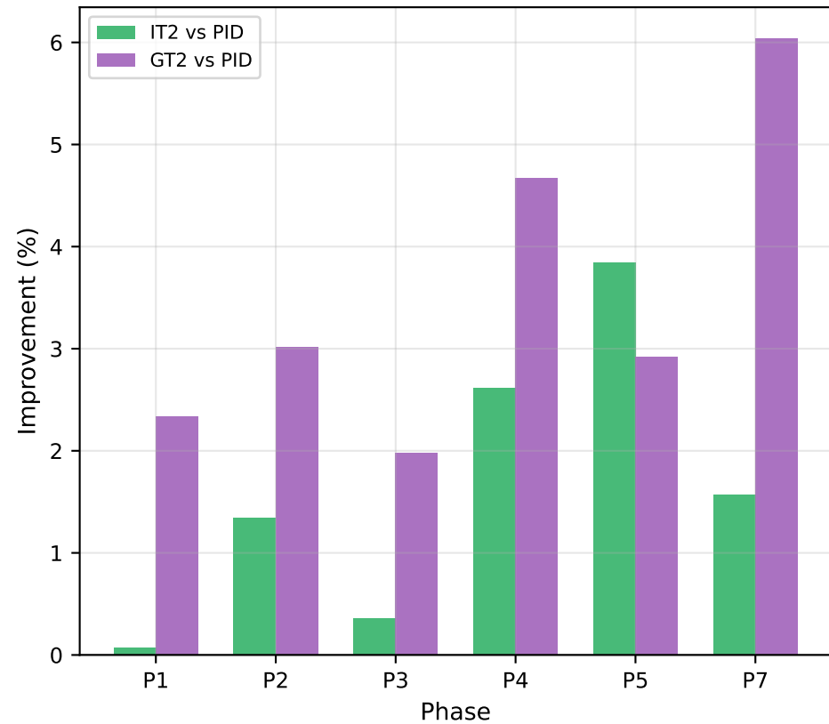
Fuzzy Controllers Improvement over PID
