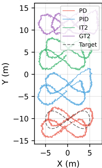
2D Trajectory (Top View) - Phase 1
