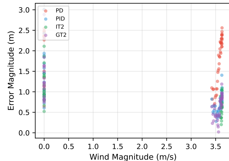
Wind vs Error Correlation - Phase 3
