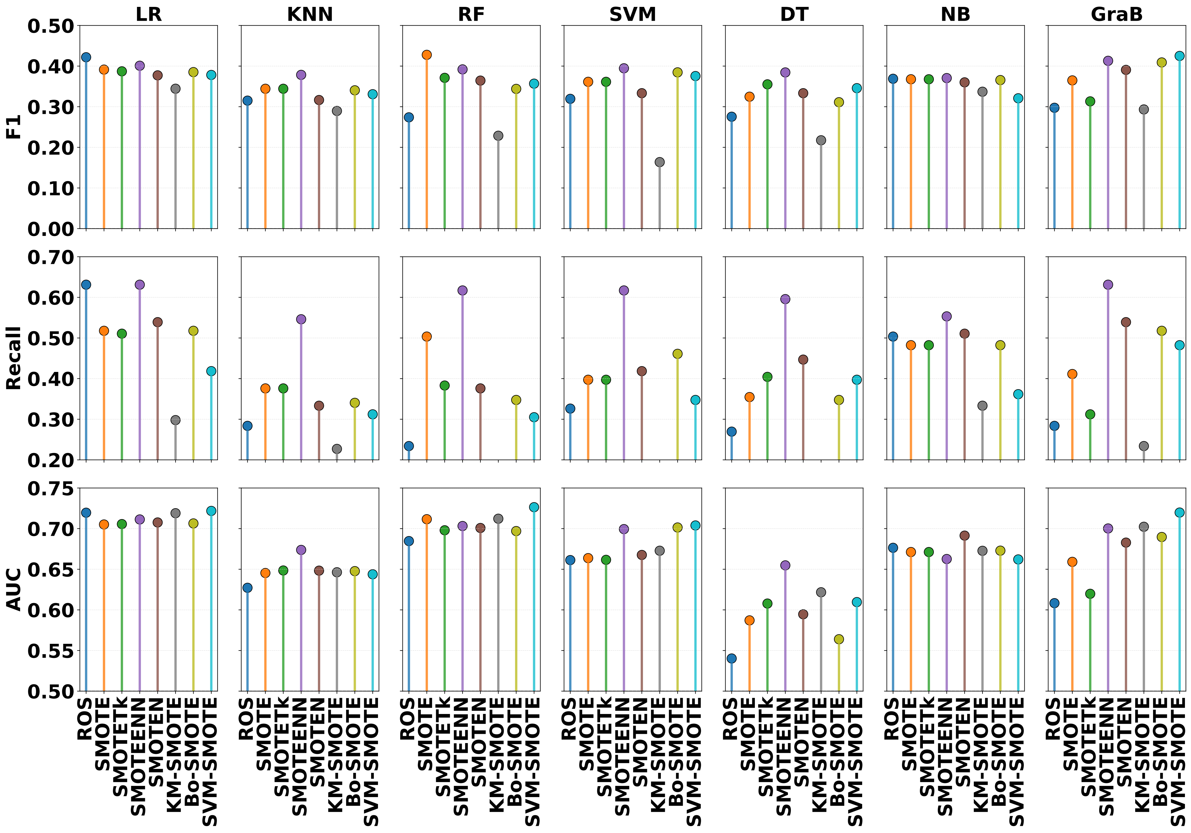
F1, Recall, and AUC-ROC Across Standard Oversampling Strategy_Riscanvi
