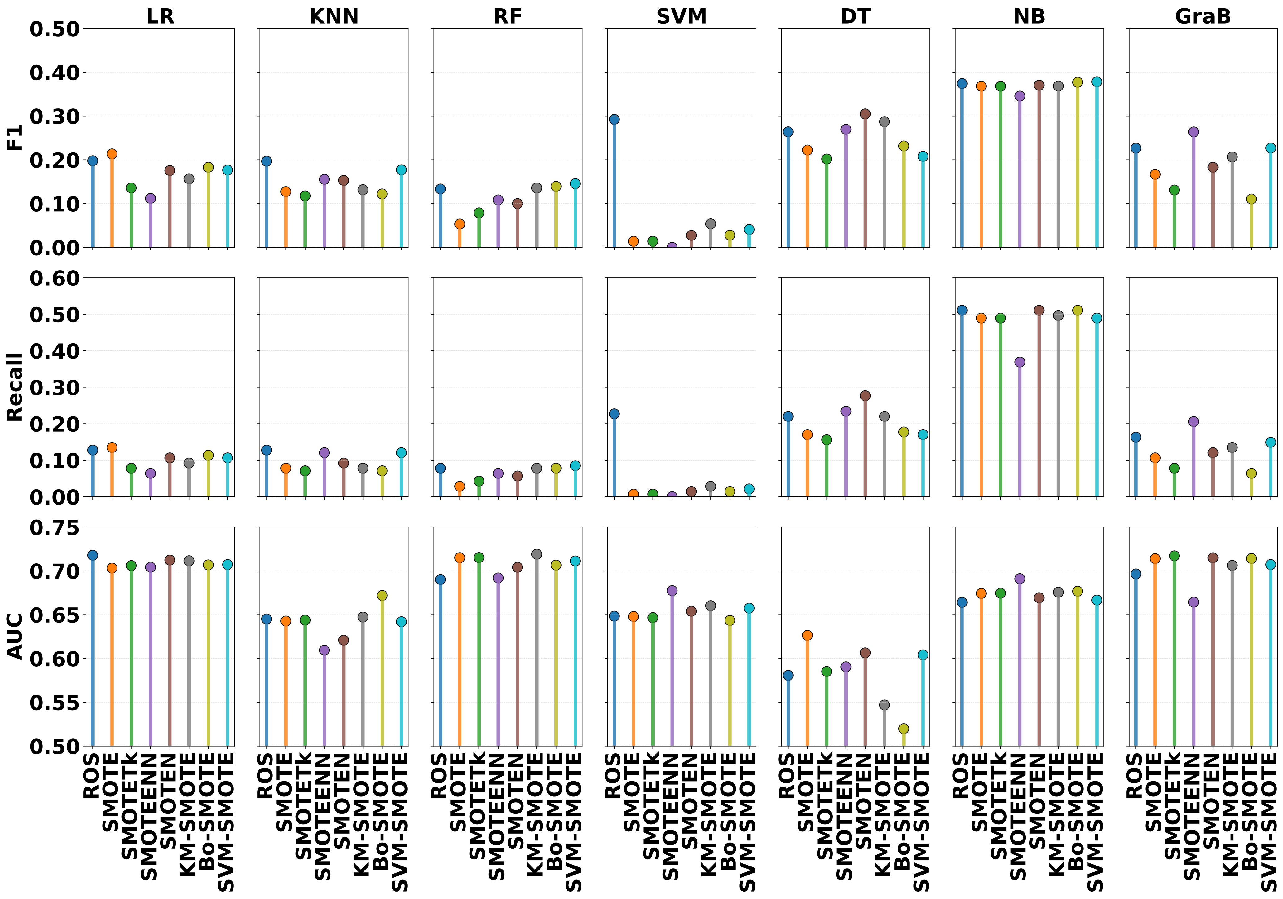
F1, Recall, and AUC-ROC Across Sensitive Attributes Strategy_Riscanvi
