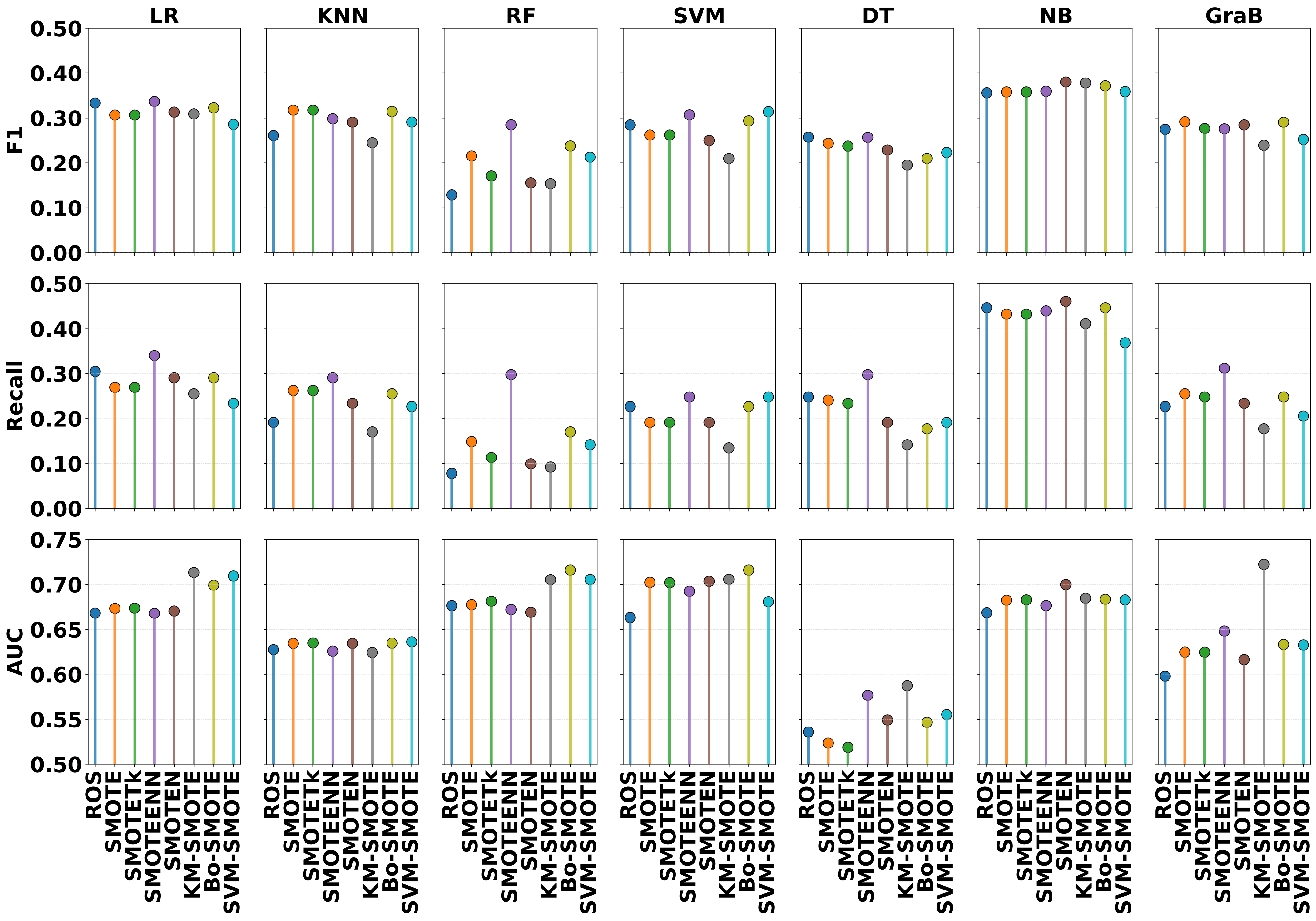
F1, Recall, and AUC-ROC Across Equalized Discriminated Group Instances_RisCanvi
