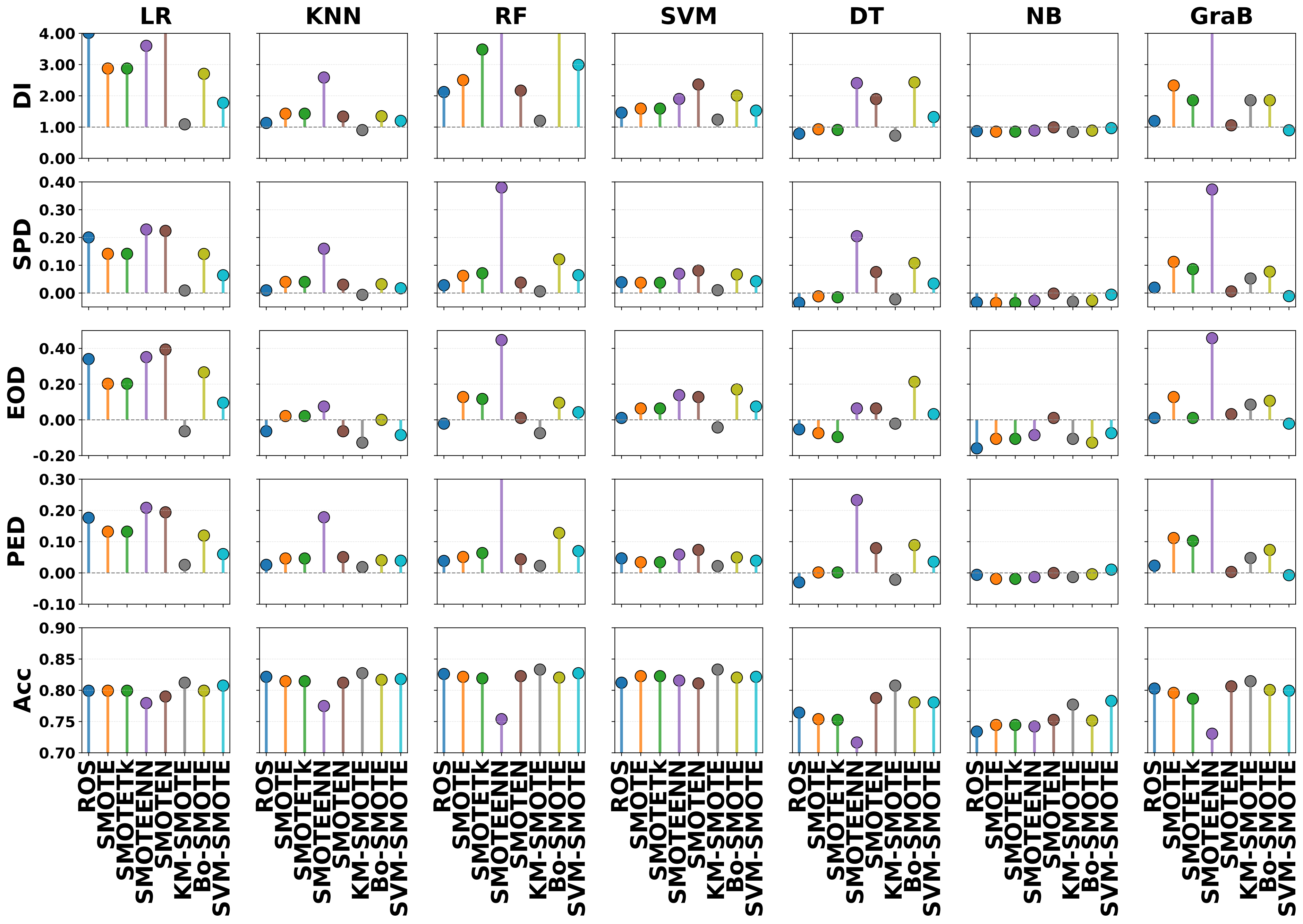
Equalized Discrimination Group Instances Strategy_RisCanvi
