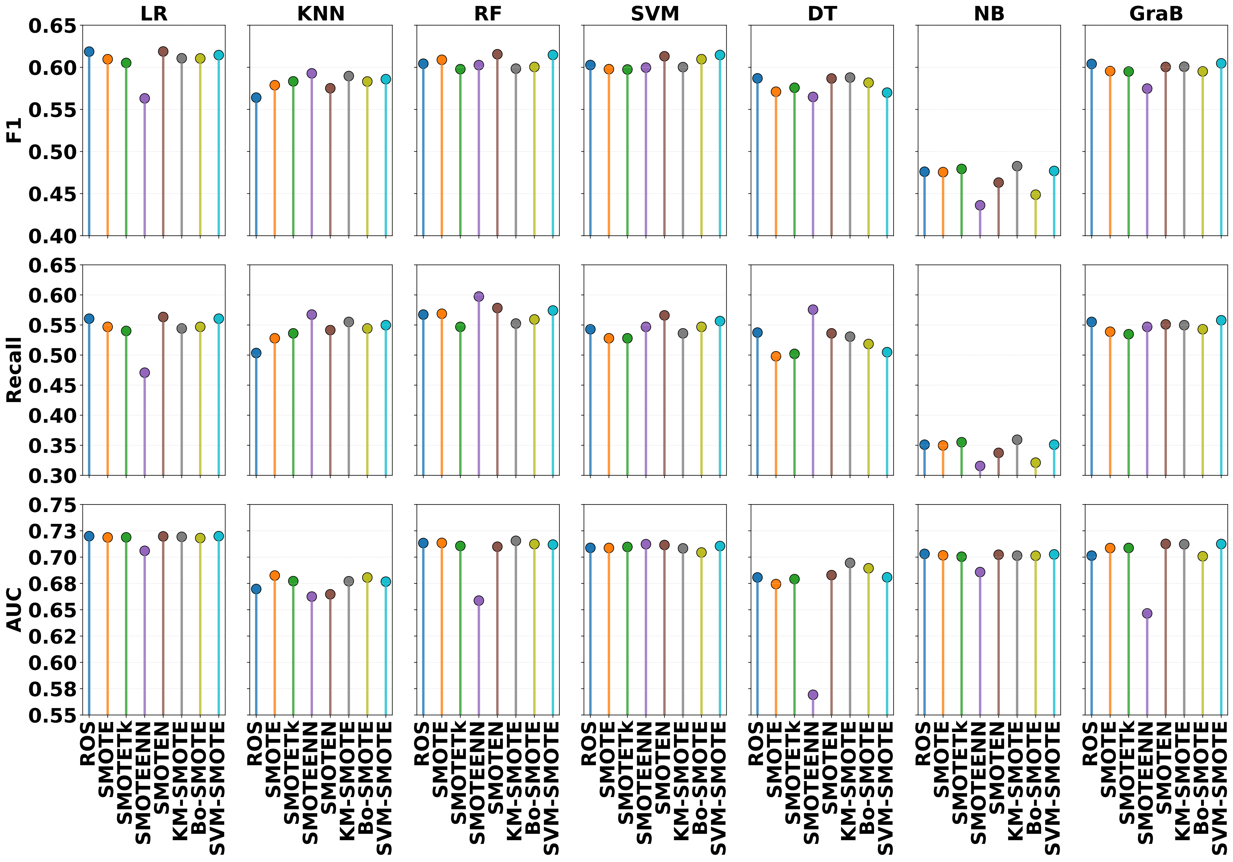
F1, Recall, and AUC-ROC Across Sensitive Attributes Strategy_COMPAS
