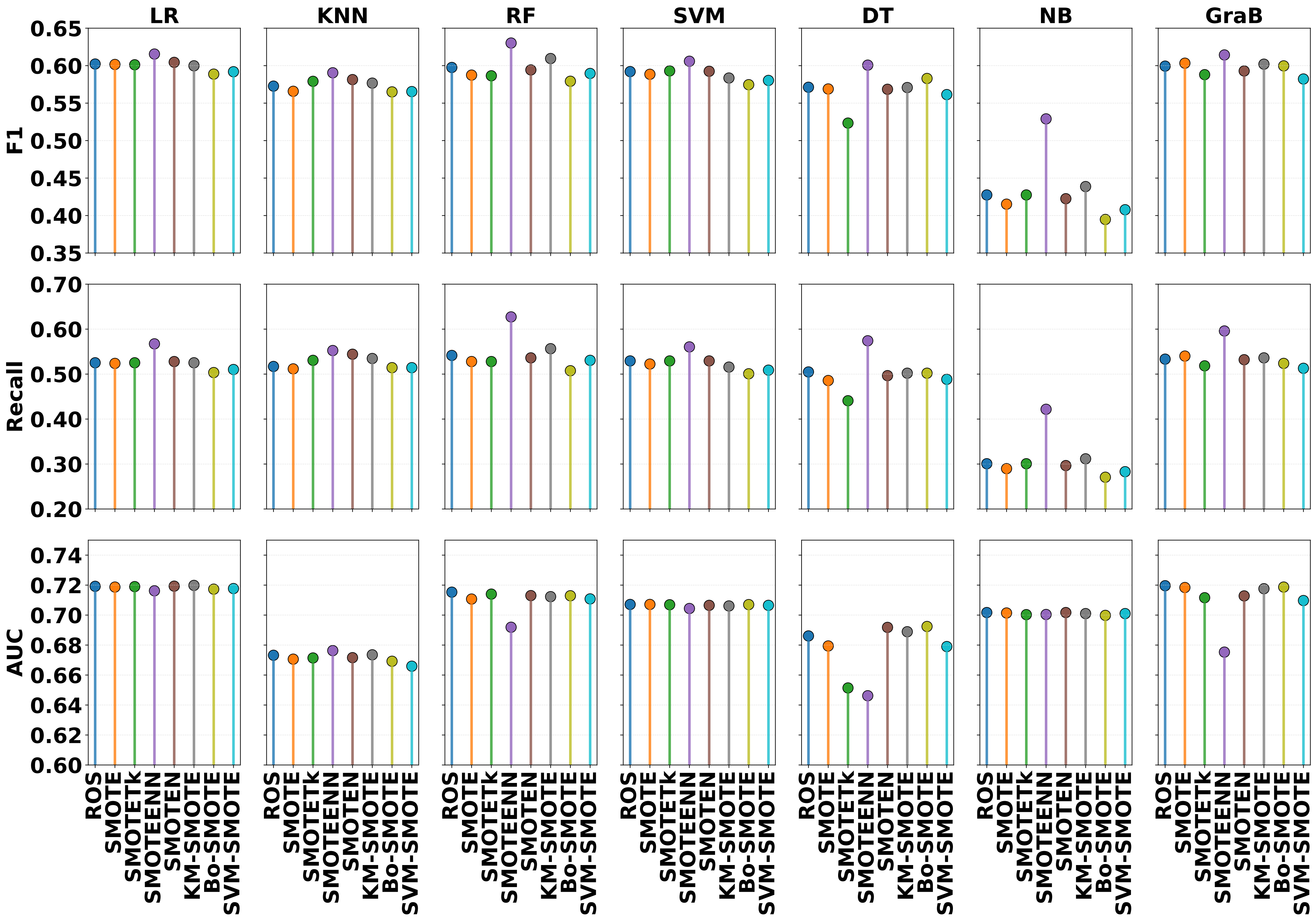
F1, Recall, and AUC-ROC Across Equalized Discriminated Group Instances_COMPAS
