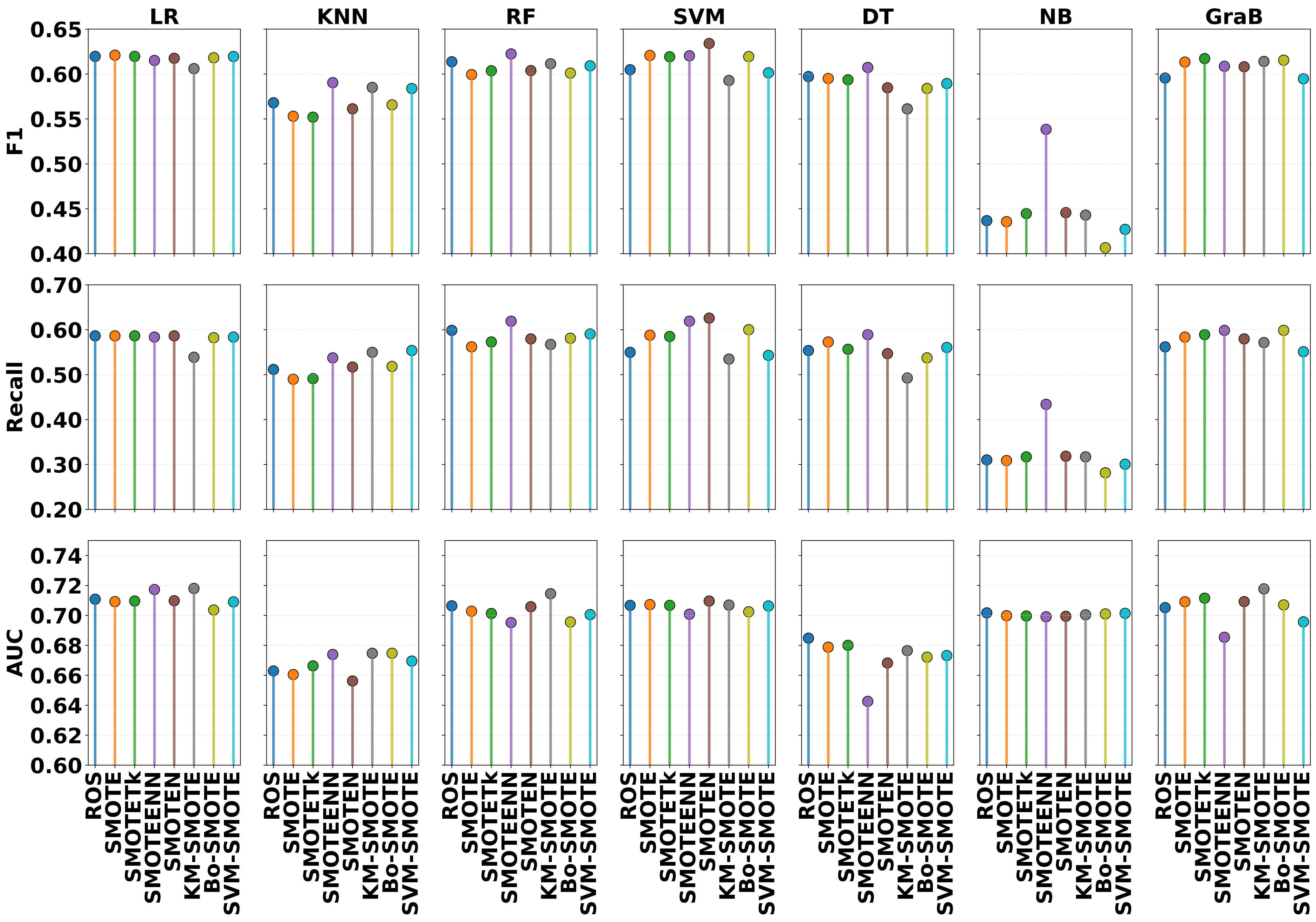
F1, Recall, and AUC-ROC Across Equalized Desired Outcomes Across Group_COMPAS
