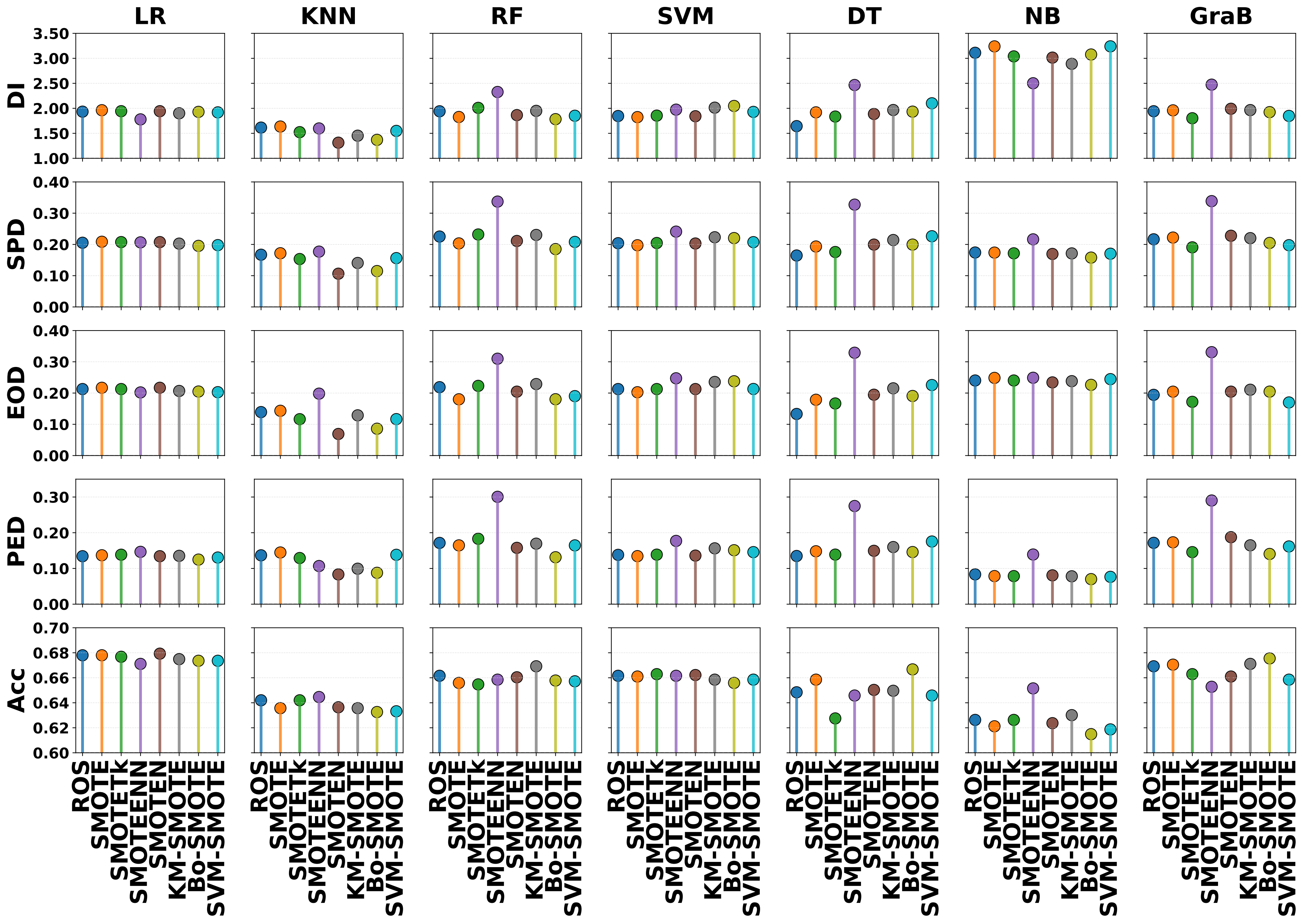
Equalized Discrimination Group Instances Strategy_COMPAS
