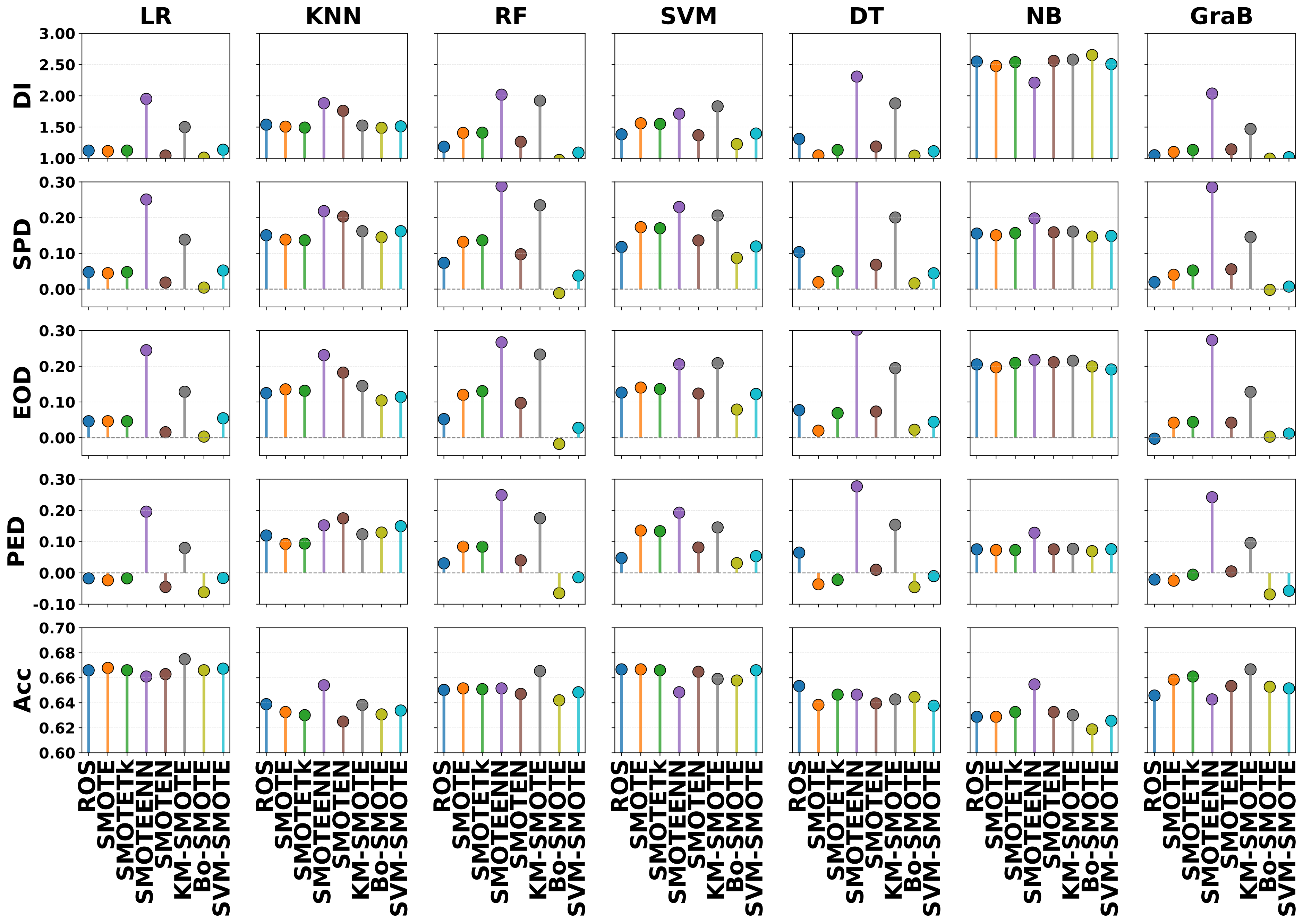
Equalized Desired Outcomes Across Group Strategy_COMPAS
