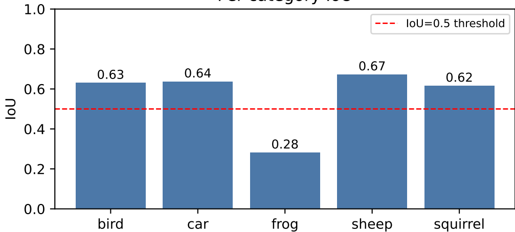
Per-category IoU
