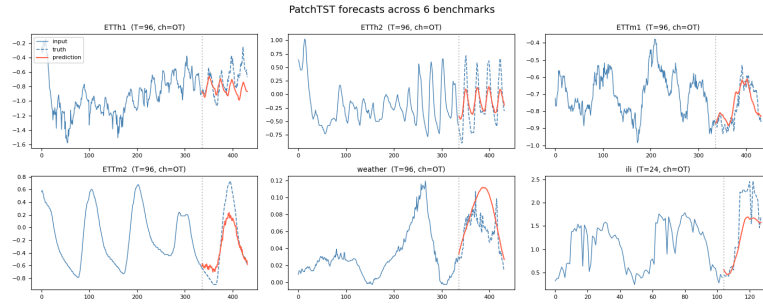
Figure 5. Predictions across 6 datasets using our PatchTST model
