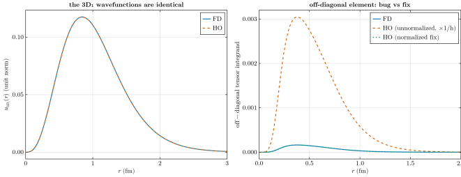
Figure 10: The off-diagonal normalization bug for the strange ^3S_1 - ^3D_1 tensor coupling. Left: the ^3D_1 reduced waves are identical in both bases. Right: the off-diagonal integrand — FD (blue), the unnormalized HO element inflated by 1/h (orange, the bug), and the normalization-invariant HO element (green), which overlaps FD.
