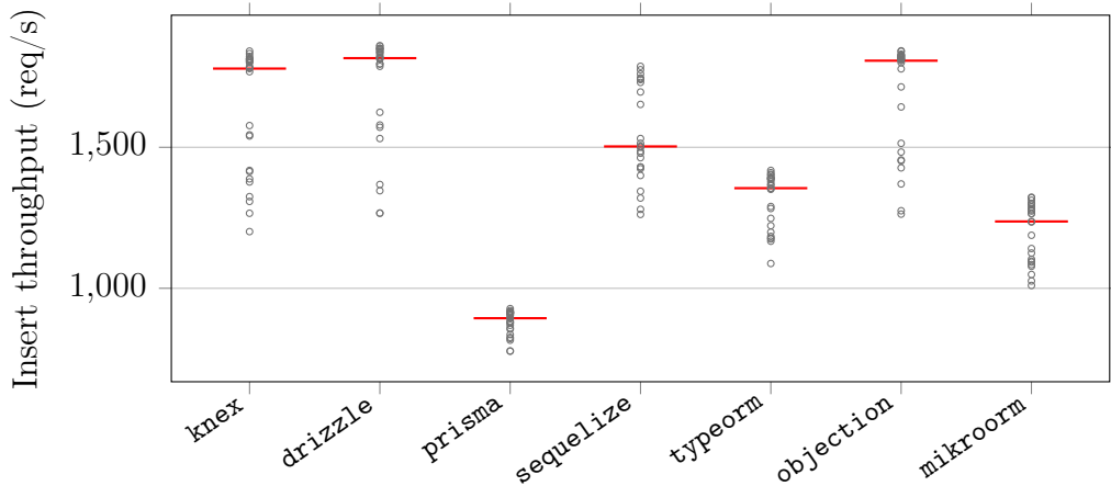
Figure 2: Corrected-state raw per-replicate MySQL insert throughput for the seven portable layers (25 independent repetitions; red bar = median; maximum CV 13.6%). The points, rather than only medians and intervals, expose any mixture or tail structure. Historical insert samples affected by the reset defect are not used for the corrected ordering.
