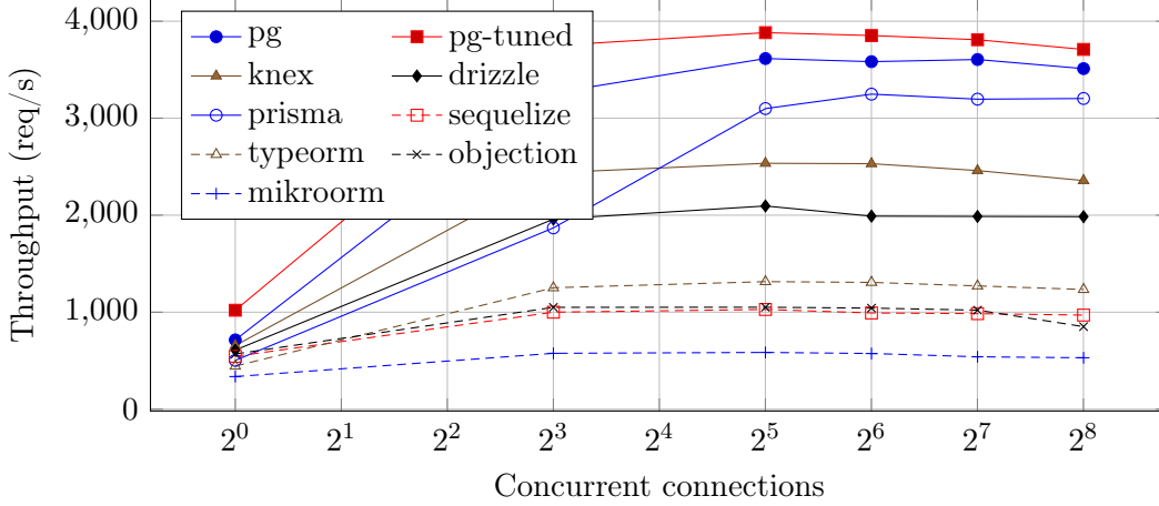
Figure 1: Throughput of each access layer on the deep/nested fetch as concurrency increases (postgres). The three-band ordering (native and tuned-native with Prisma on top, query builder and lightweight ORM in the middle, data-mapper ORMs below) holds at 32 connections and above; at 1 and 8 connections Prisma is mid-pack (Section 4).
