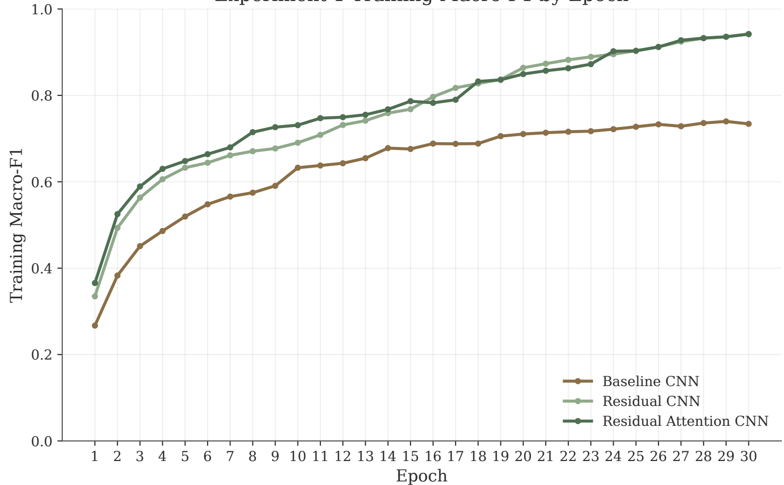
Experiment 1 Training Macro-F1 by Epoch
