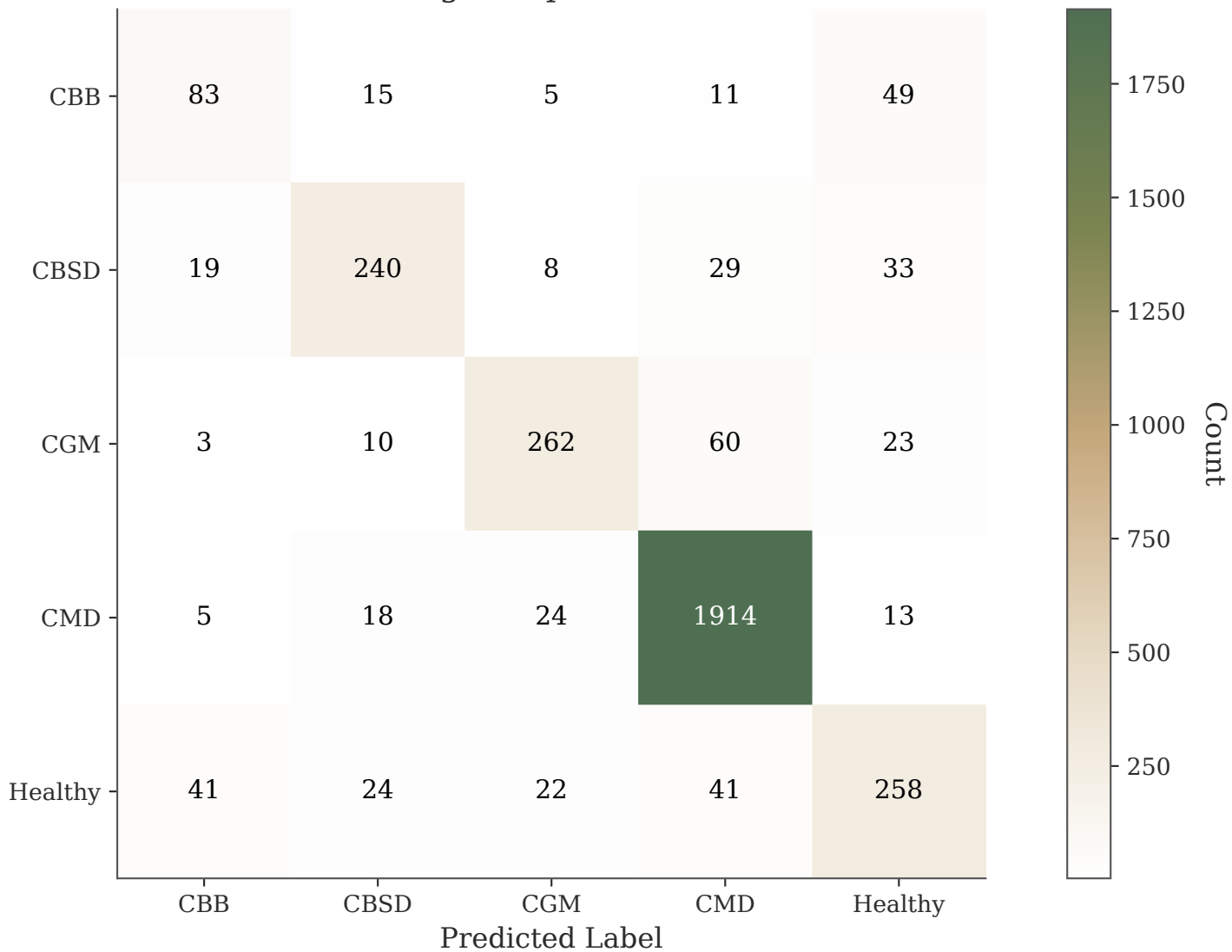
Final Winning Setup: Confusion Matrix
