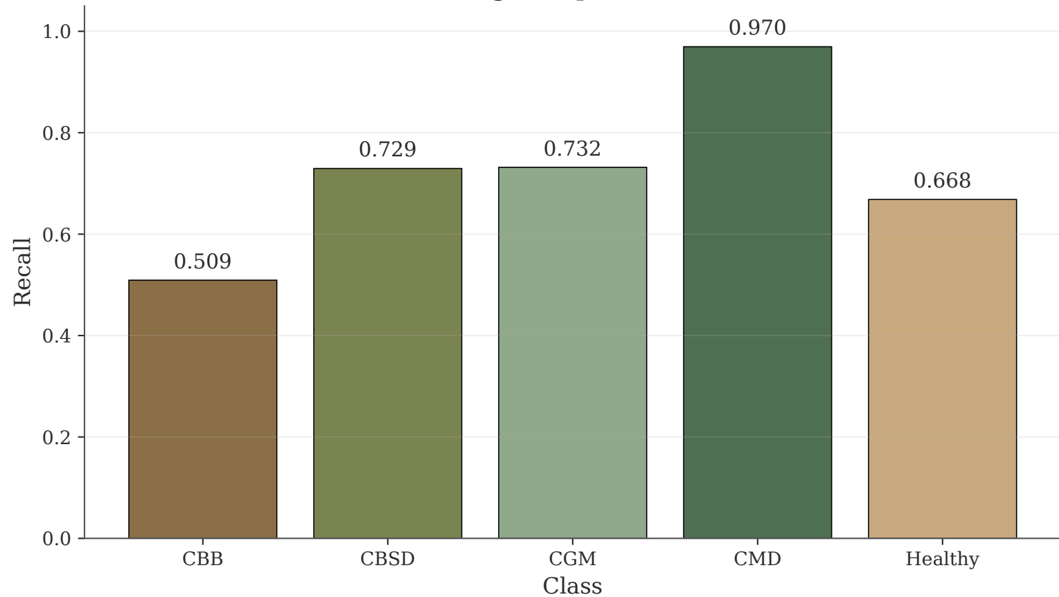
Final Winning Setup: Per-Class Recall
