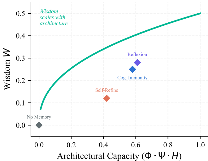
(b) Second Law: W \propto \Phi^\alpha \cdot \Psi^\beta \cdot H^\gamma
