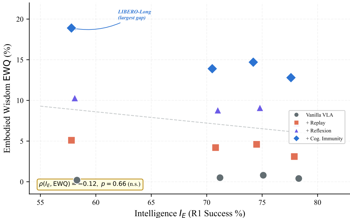
IW Decorrelation on LIBERO: Each Point = Agent \times Suite
