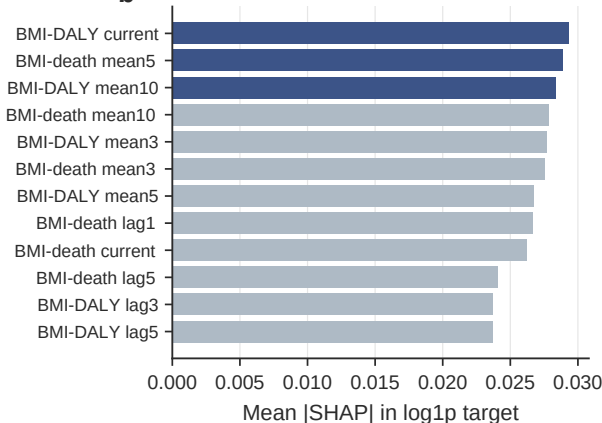
b Top features: DALY 5-y tree
