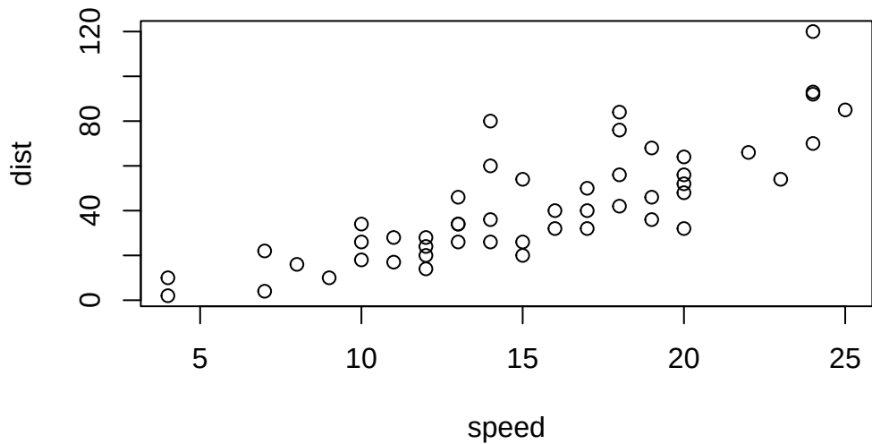
Cars dataset
