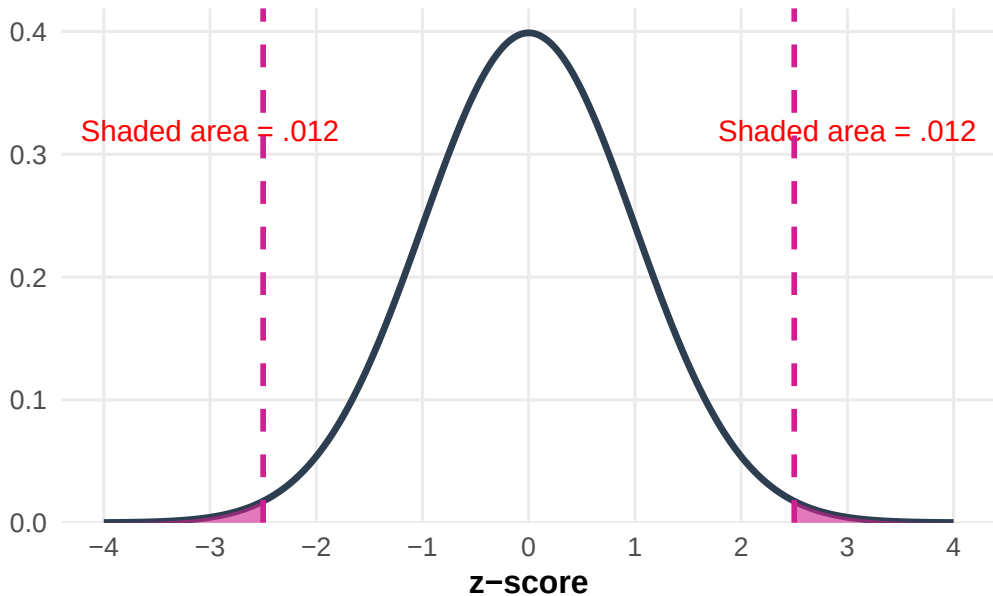
Plot of z distribution showing corresponding areas
