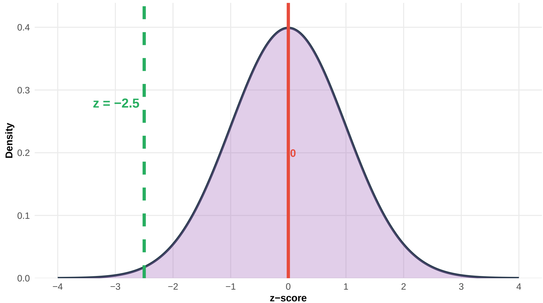
Standard Normal Distribution (Z-distribution)
