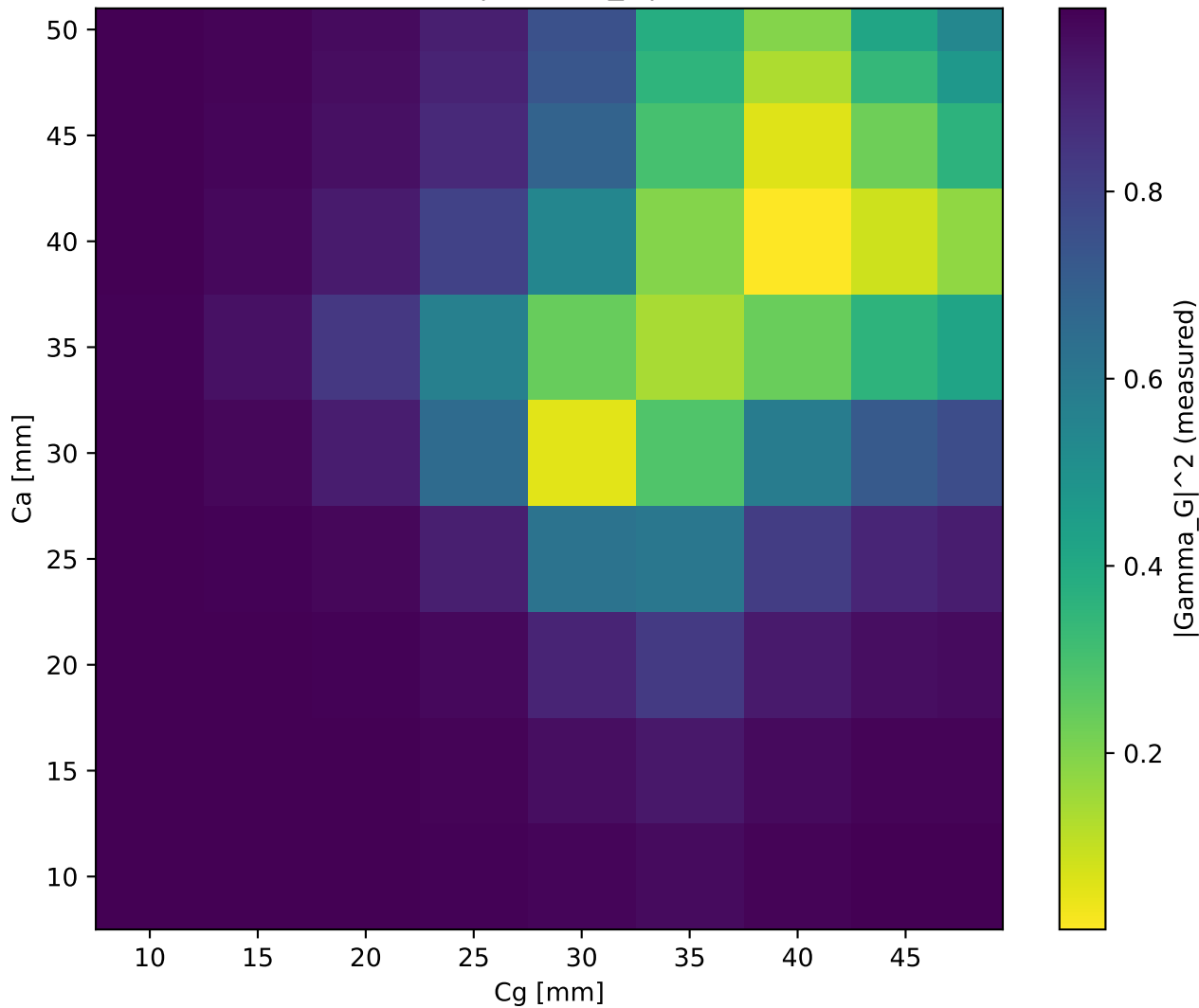
Measured map of |\text{Gamma\_G}|^2 at 38.0 MHz
