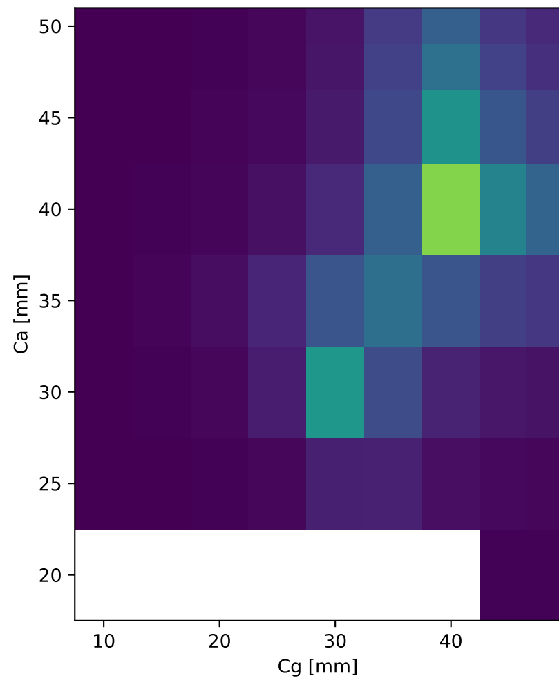
Measurement (VNA)
