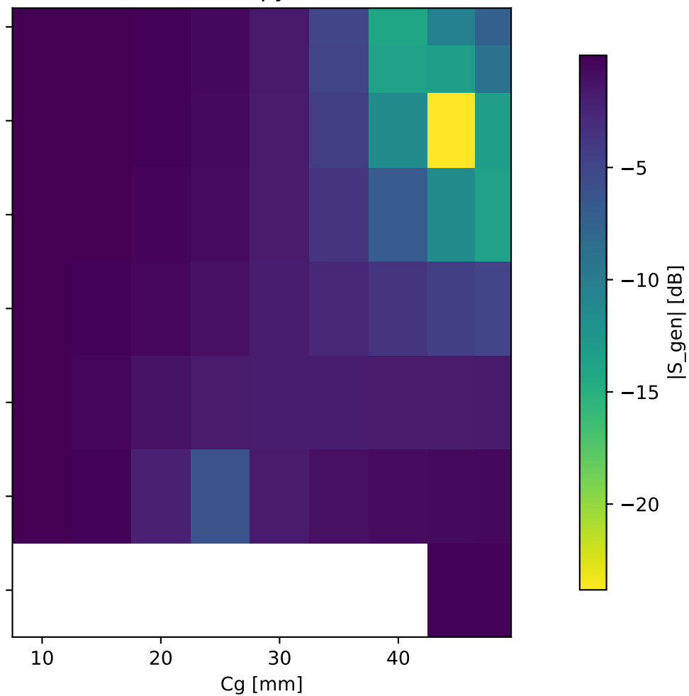
Model (pyRFtk)
