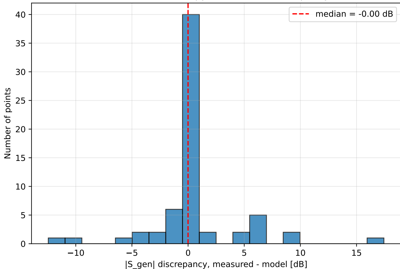
Distribution of the pyRFtk vs VNA discrepancy
