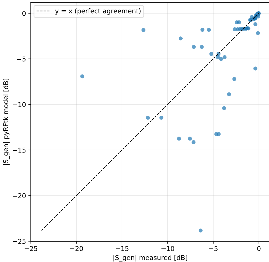
Parity: pyRFtk vs VNA
