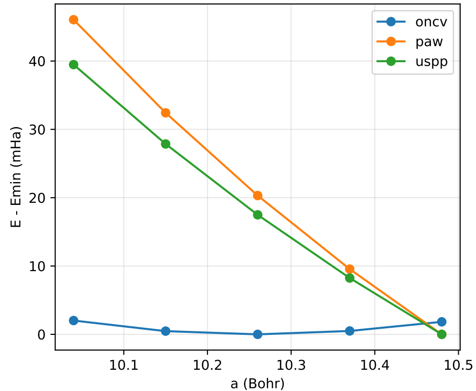
CoQui-native (broken)
