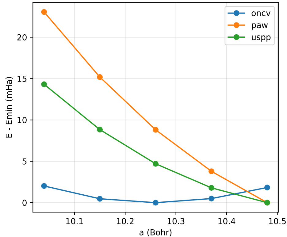
QE 1e-substitution
