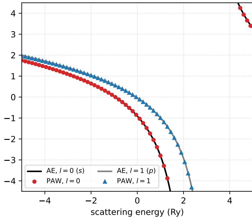
(b) l = 0, 1 ( s, p ): projectors present
