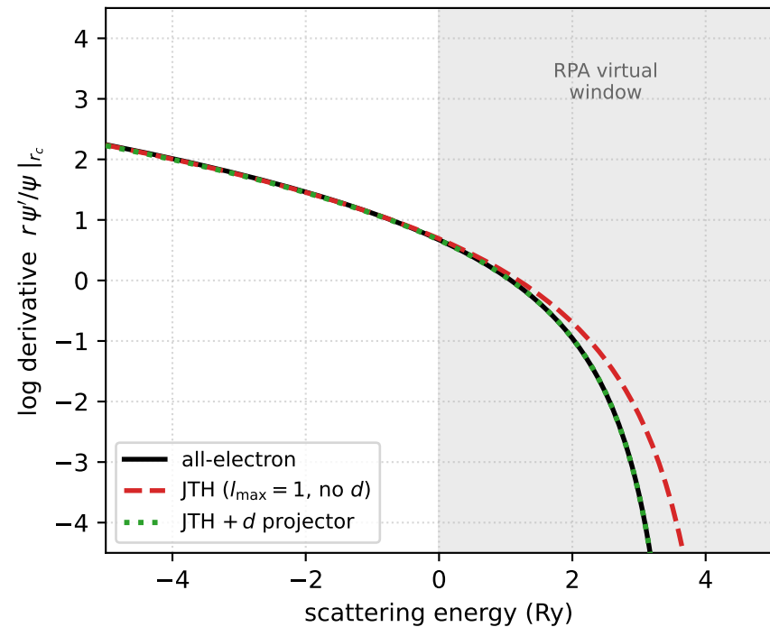
(a) l = 2 ( d ) channel
