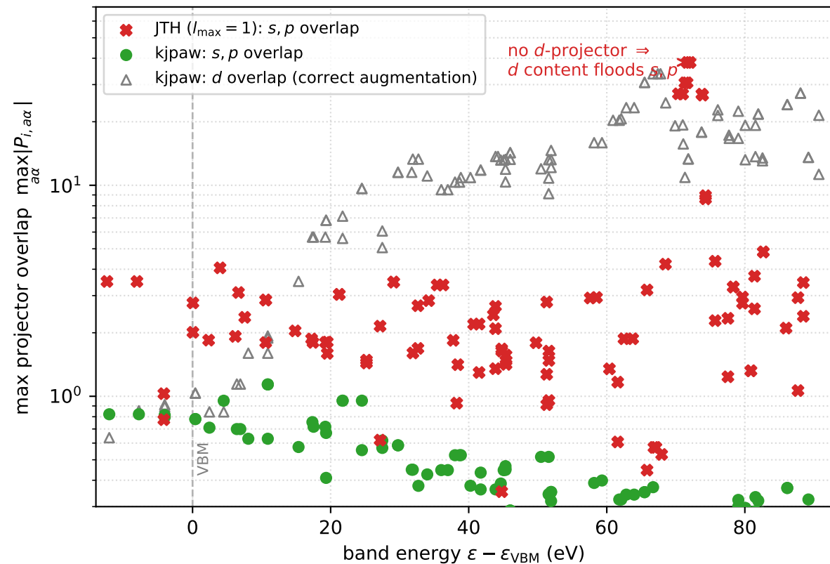
Si 4 \times 4 \times 4 , N_b = 100 : projector amplitude vs band energy
