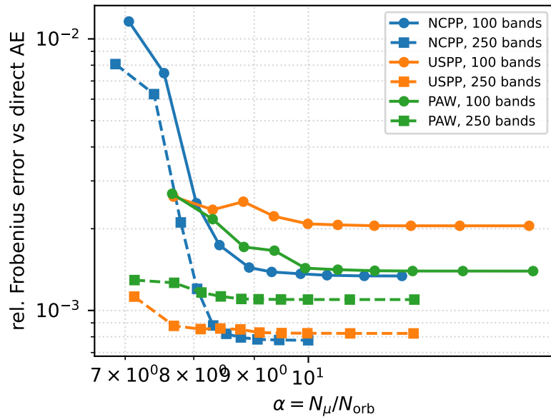
exchange V_x
