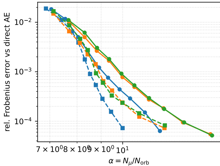
Hartree V_H
