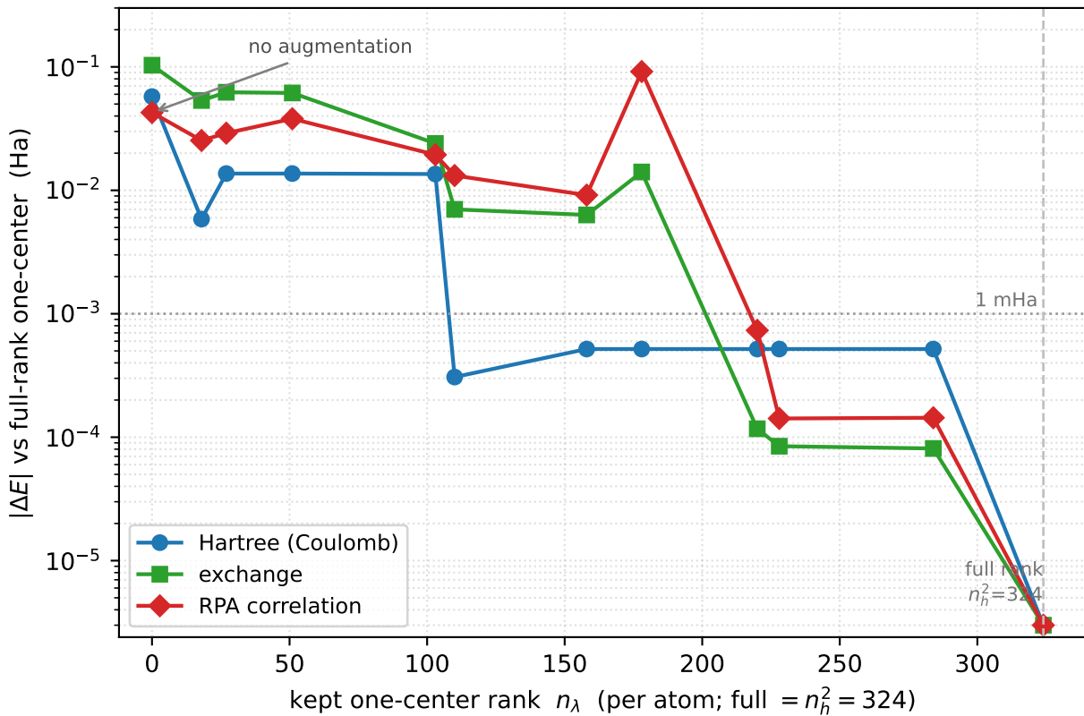
Si kjpaw, 3 \times 3 \times 3 , N_b = 100 : one-center compression error
