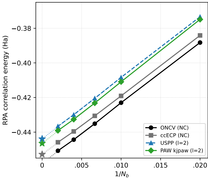
Si, 6×6×6 k-grid
