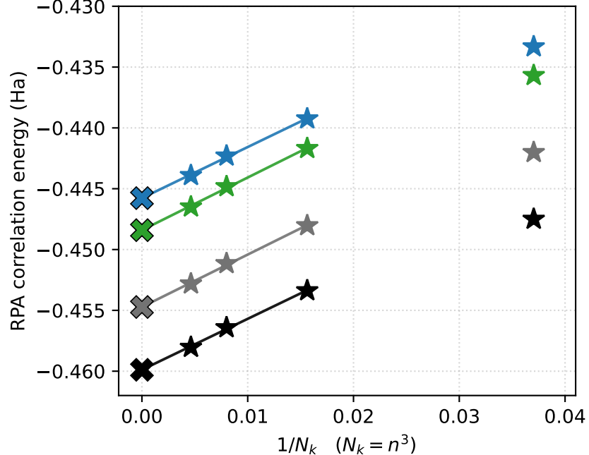
(b) k -point convergence, N_b \rightarrow \infty
