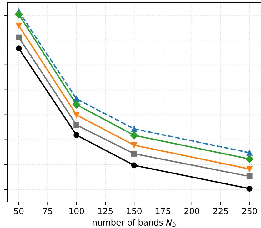
Si, 4×4×4 k-grid
