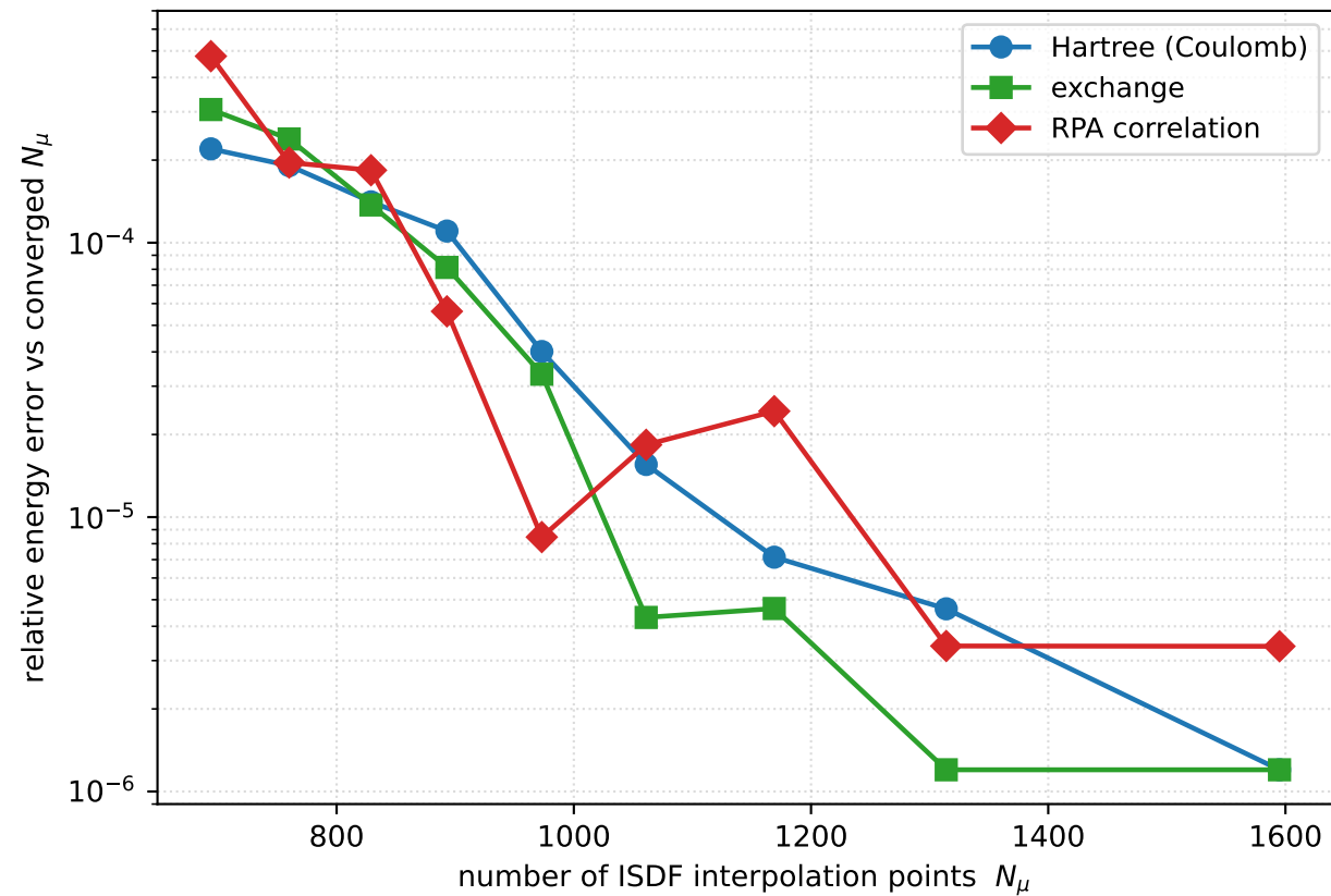
ZnO (kjpaw, Zn semicore 3d), 3 \times 3 \times 3 , N_b = 100
