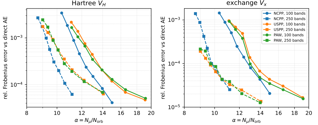
FIG. 1. Relative Frobenius error of the tensor-hypercontracted Hartree (left) and exchange (right) matrix elements versus the number of ISDF interpolation points N_\mu , for LiH on a 2 \times 2 \times 2 mesh with norm-conserving (NCPP), ultrasoft (USPP), and projector-augmented-wave (PAW) pseudization. Tightening the ISDF threshold from 3 \times 10^{-2} to 10^{-6} drives the error down by about two and a half orders of magnitude. PAW converges at the same rate as the ultrasoft case (the two curves overlap), while the norm-conserving case reaches a given accuracy at smaller N_\mu because it carries no compensation charges.
