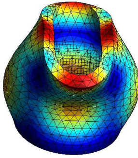
Figure 16.12: Typical mode shape of a sleeve
