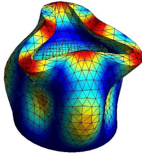
Figure 16.13: Typical mode shape of a sleeve
