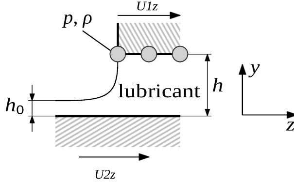
Figure 16.4: assumptions for partially flooded boundaries of the bearing
